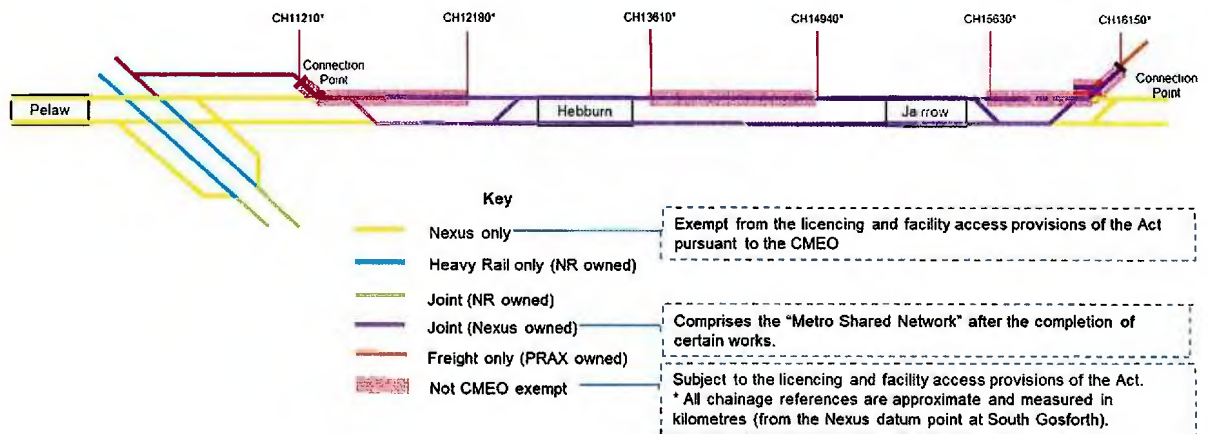
Diagram 2 – Metro Shared Network (as anticipated following completion of works)
